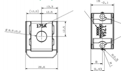
Dimensions [mm]
